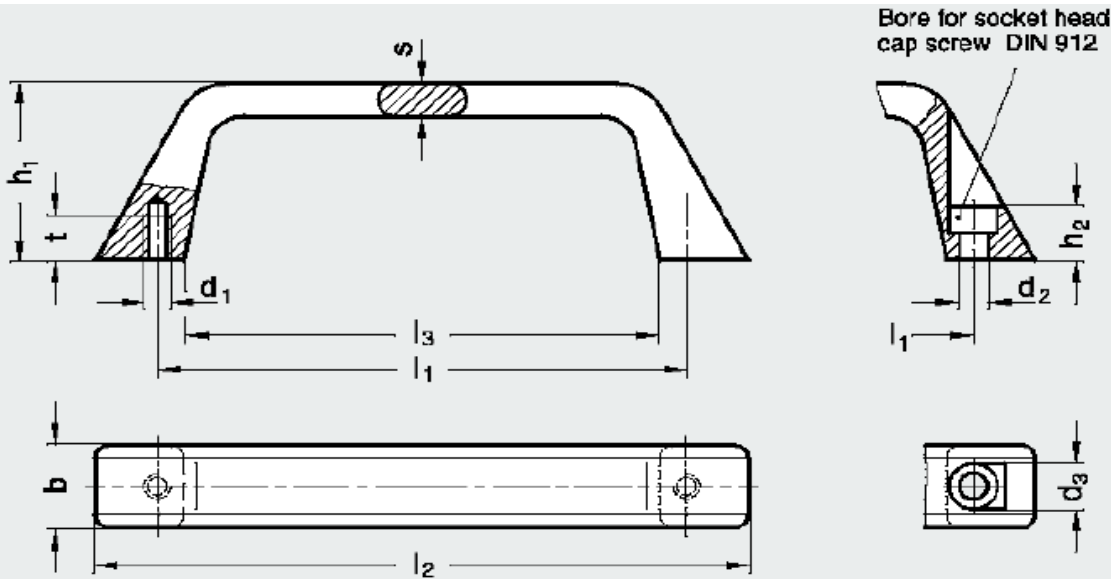
Type A mounting from the back
